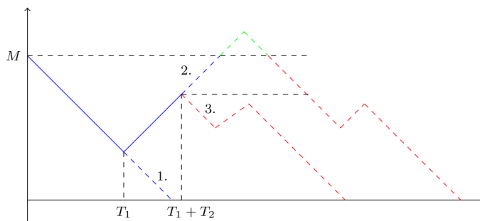
Fig. 2. The three different types of paths from (M, -1) to (0, +1) .
